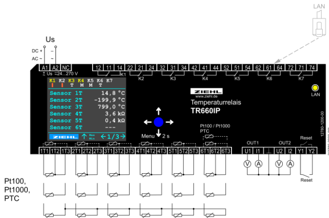
TR660IP Analog
